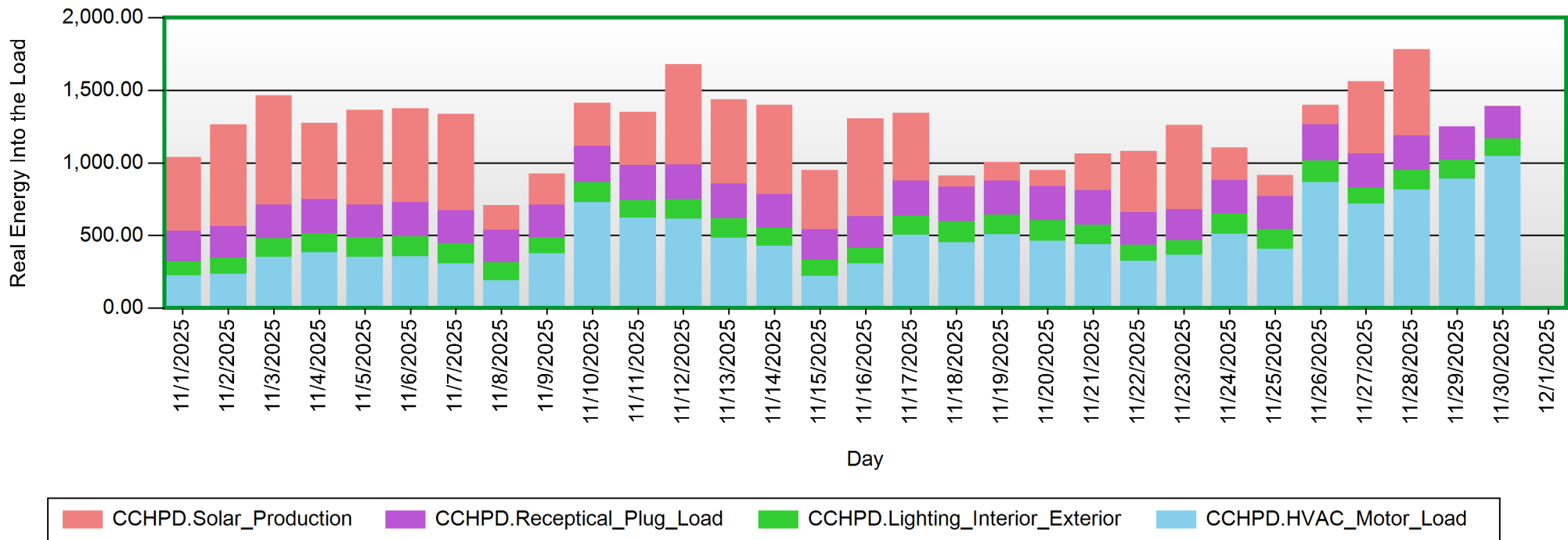
Energy Usage 00:00 - 00:00
